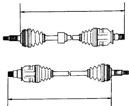
Fig. 5: Measuring Axle Shaft Standard Length (Celica FWD) Courtesy of Toyota Motor Sales, U.S.A., Inc.
